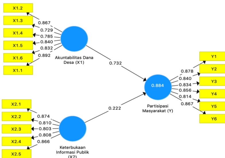
Gambar 2. PLS Algoritma
